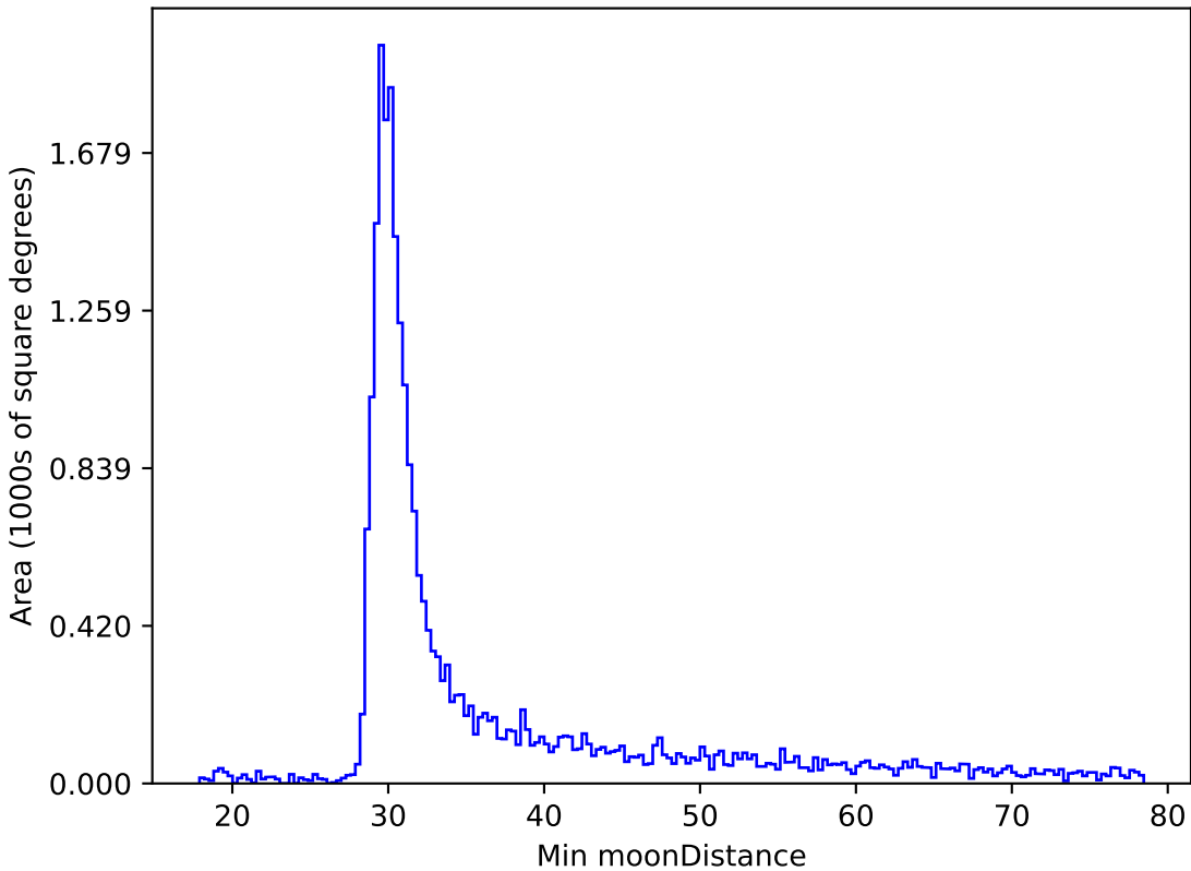
too_combined_s0.5_v3.4_10yrs All sky i band: Min moonDistance
