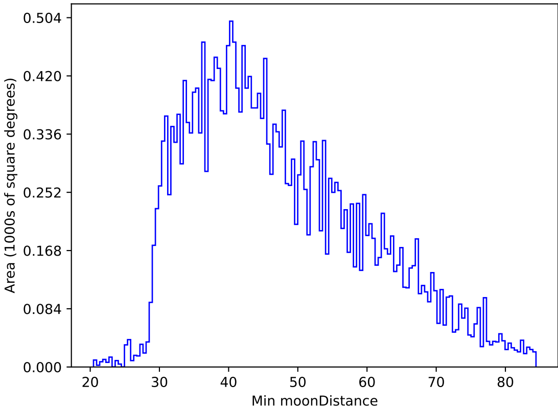
too_combined_s0.5_v3.4_10yrs All sky g band: Min moonDistance
