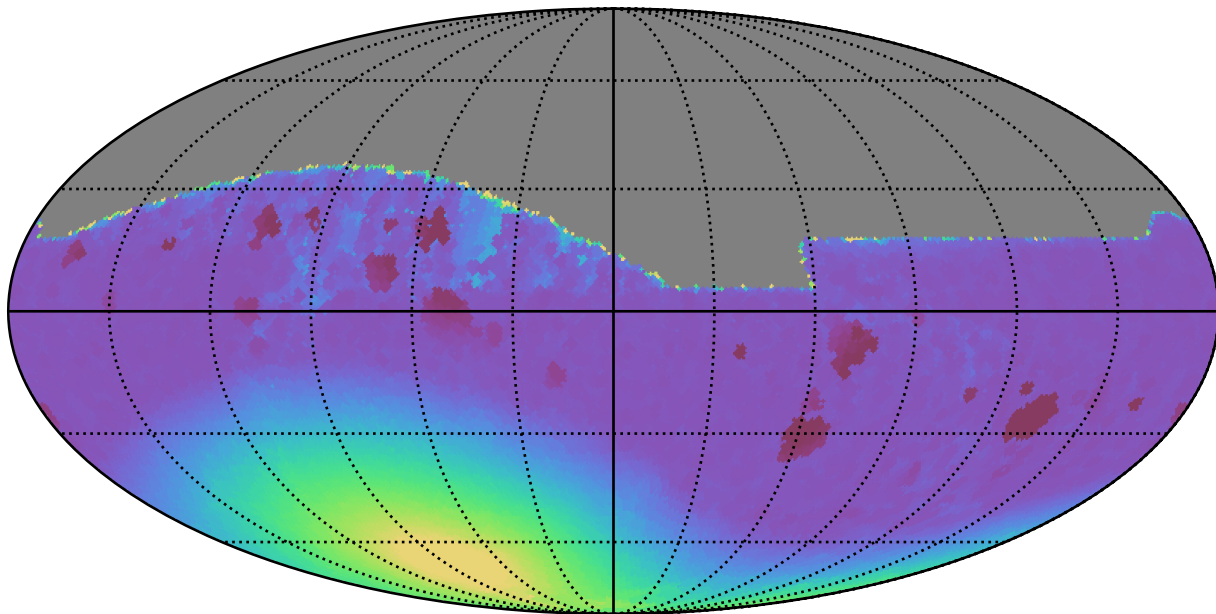
too_combined_s0.5_v3.4_10yrs All sky all bands: Min moonDistance
