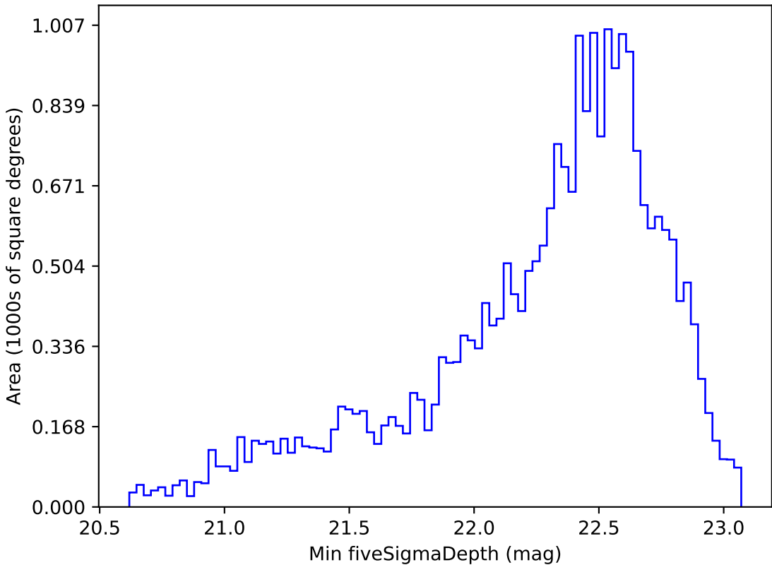
too_combined_s0.5_v3.4_10yrs Yr 1 z band: Min fiveSigmaDepth
