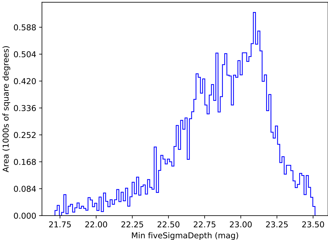
too_combined_s0.5_v3.4_10yrs Yr 1 u band: Min fiveSigmaDepth
