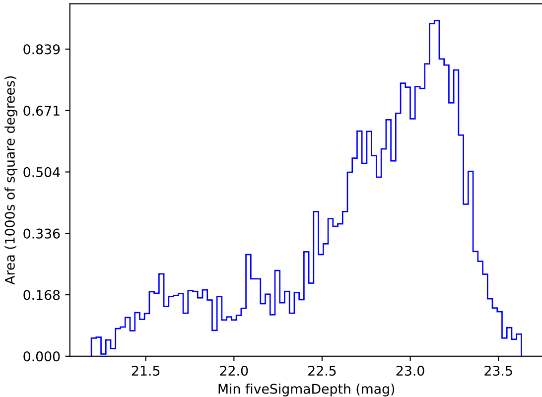
too_combined_s0.5_v3.4_10yrs Yr 1 i band: Min fiveSigmaDepth
