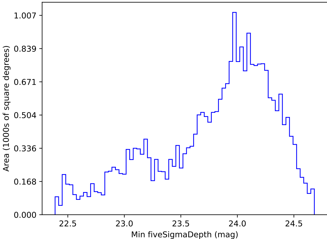
too_combined_s0.5_v3.4_10yrs Yr 1 g band: Min fiveSigmaDepth
