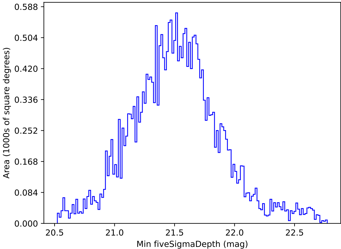
too_combined_s0.5_v3.4_10yrs Yr 1 all bands: Min fiveSigmaDepth
