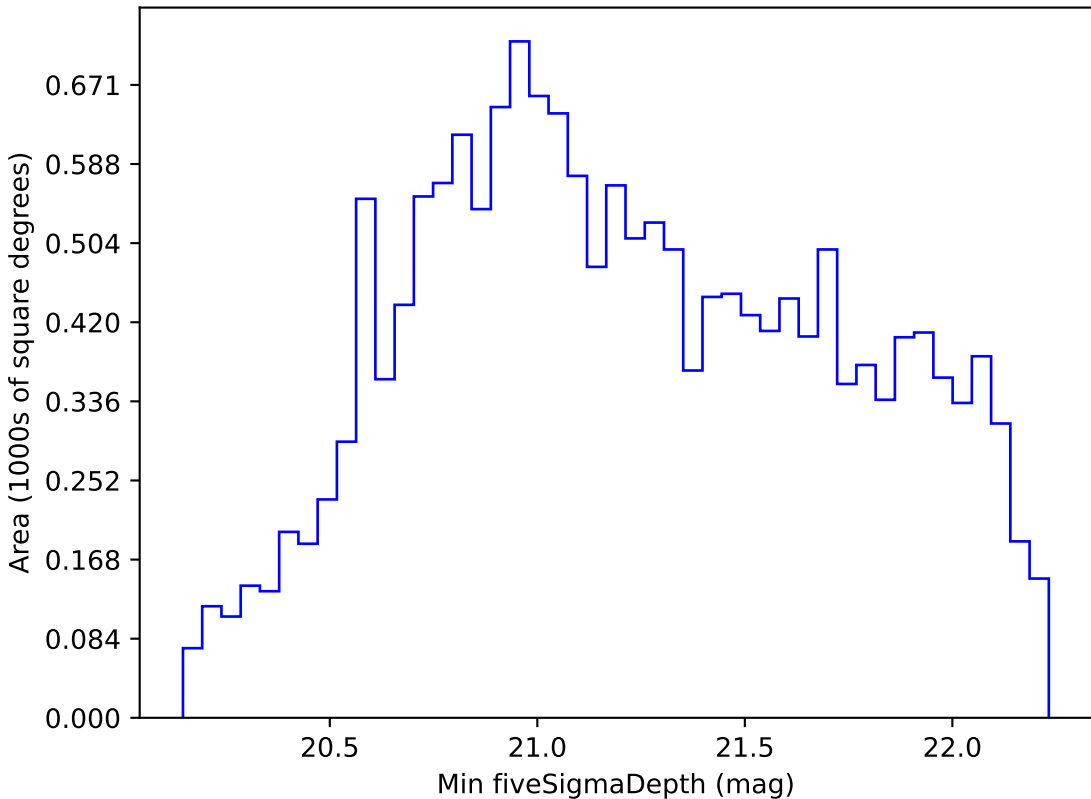
too_combined_s0.5_v3.4_10yrs WFD z band: Min fiveSigmaDepth
