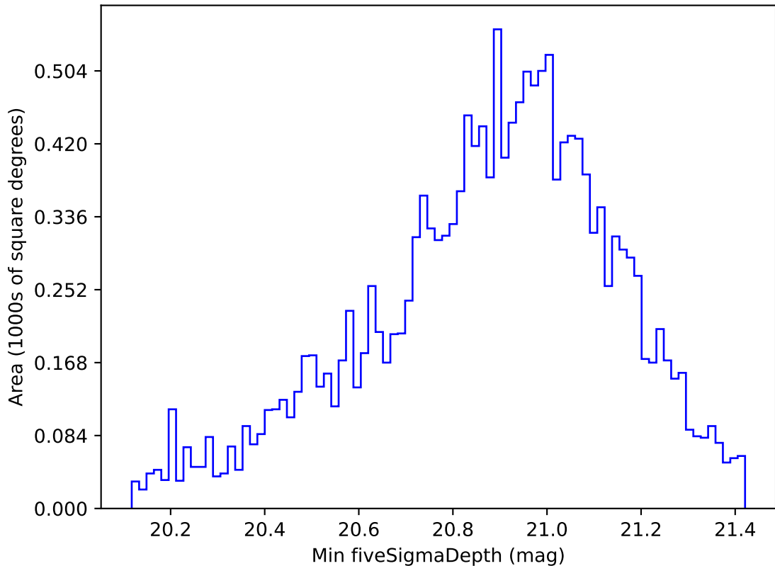
too_combined_s0.5_v3.4_10yrs WFD y band: Min fiveSigmaDepth
