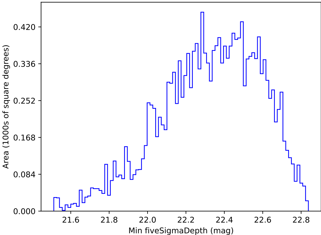
too_combined_s0.5_v3.4_10yrs WFD u band: Min fiveSigmaDepth
