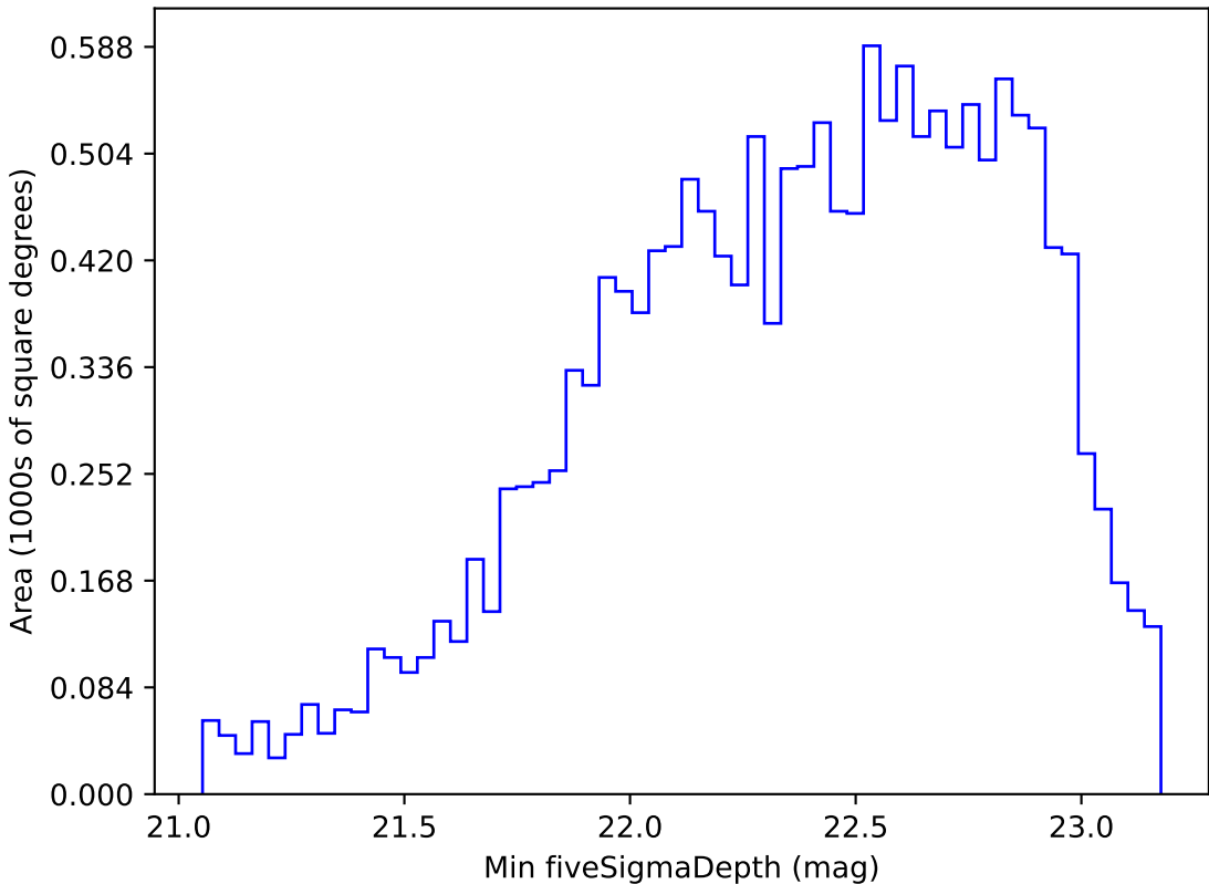
too_combined_s0.5_v3.4_10yrs WFD r band: Min fiveSigmaDepth
