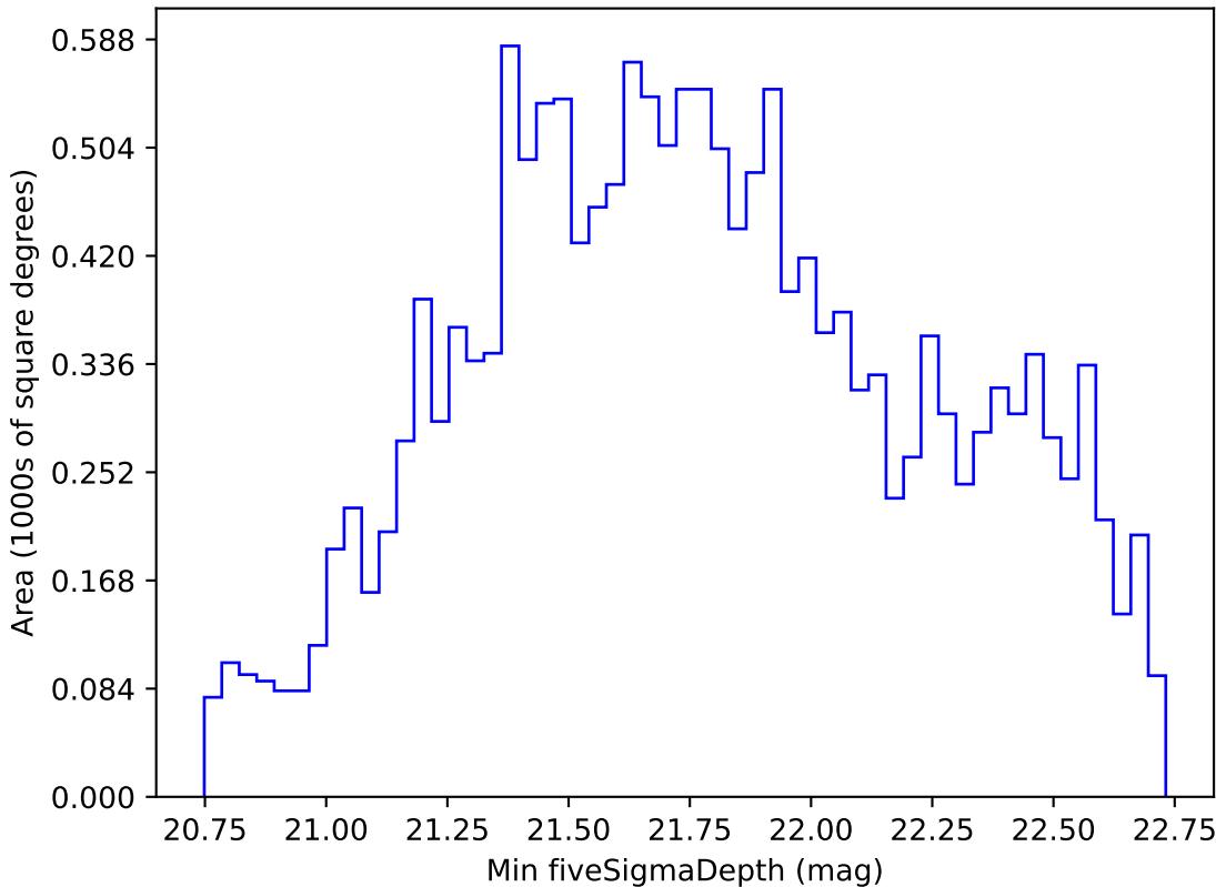
too_combined_s0.5_v3.4_10yrs WFD i band: Min fiveSigmaDepth
