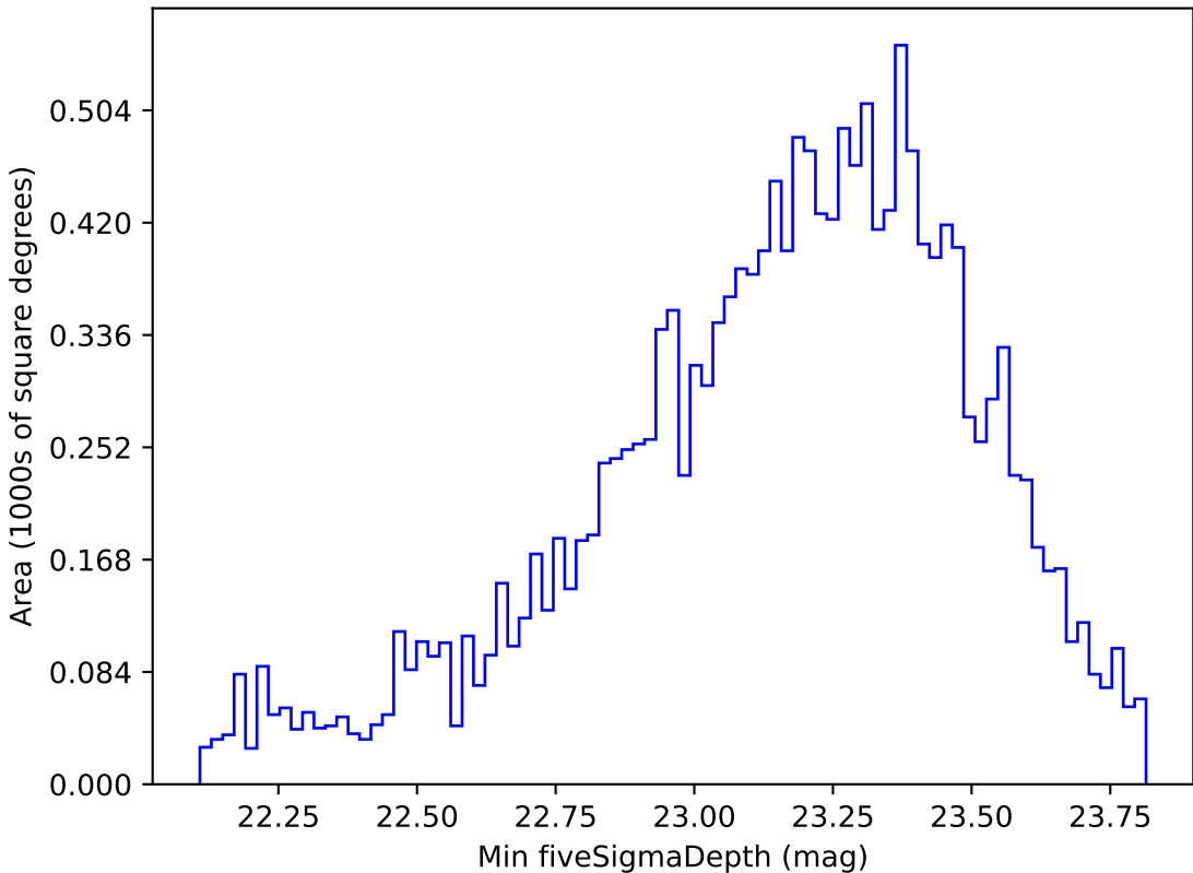
too_combined_s0.5_v3.4_10yrs WFD g band: Min fiveSigmaDepth
