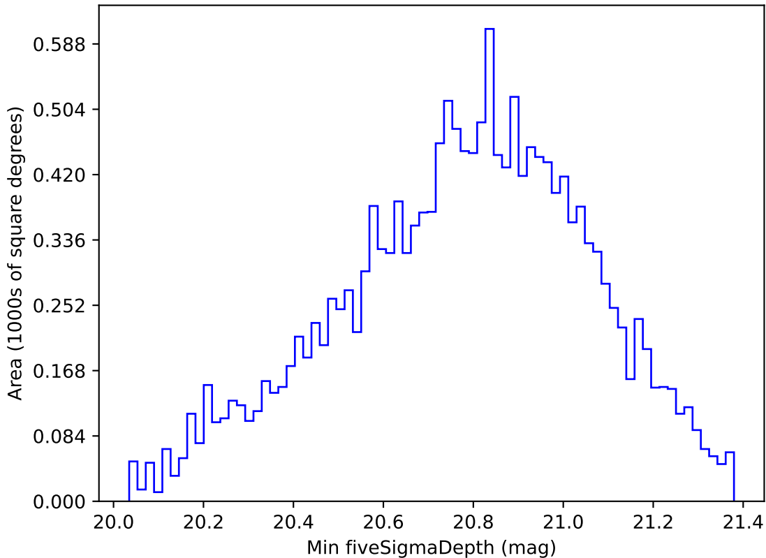
too_combined_s0.5_v3.4_10yrs WFD all bands: Min fiveSigmaDepth
