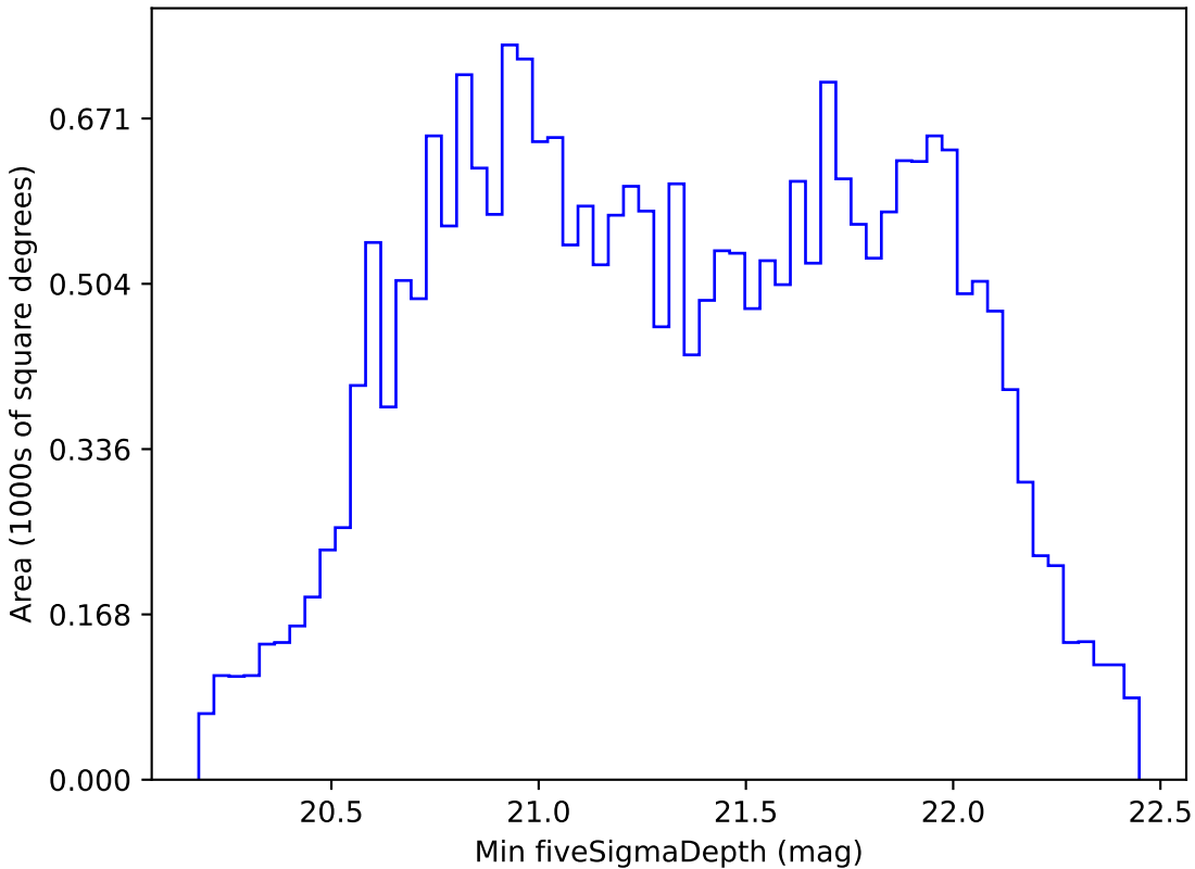
too_combined_s0.5_v3.4_10yrs All sky z band: Min fiveSigmaDepth
