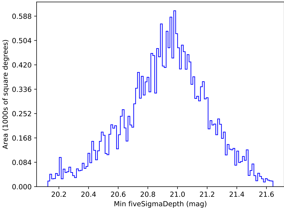
too_combined_s0.5_v3.4_10yrs All sky y band: Min fiveSigmaDepth
