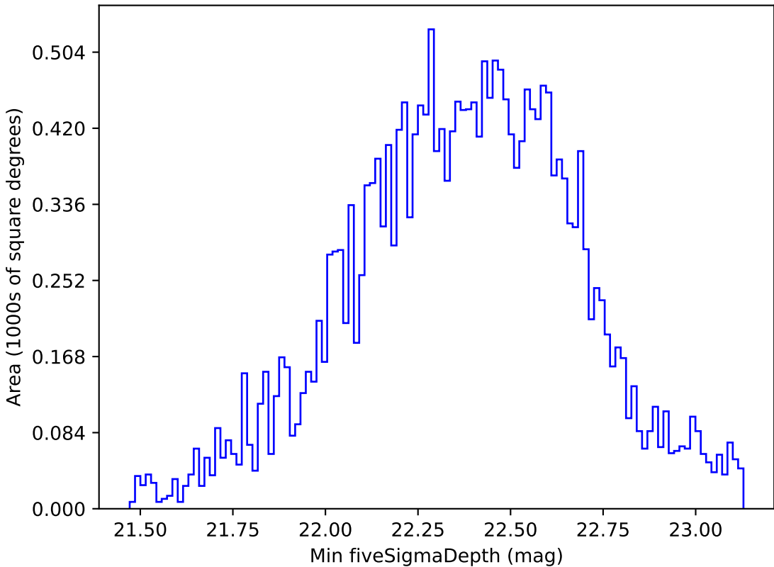
too_combined_s0.5_v3.4_10yrs All sky u band: Min fiveSigmaDepth
