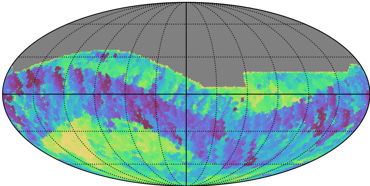
too_combined_s0.5_v3.4_10yrs All sky i band: Min fiveSigmaDepth
