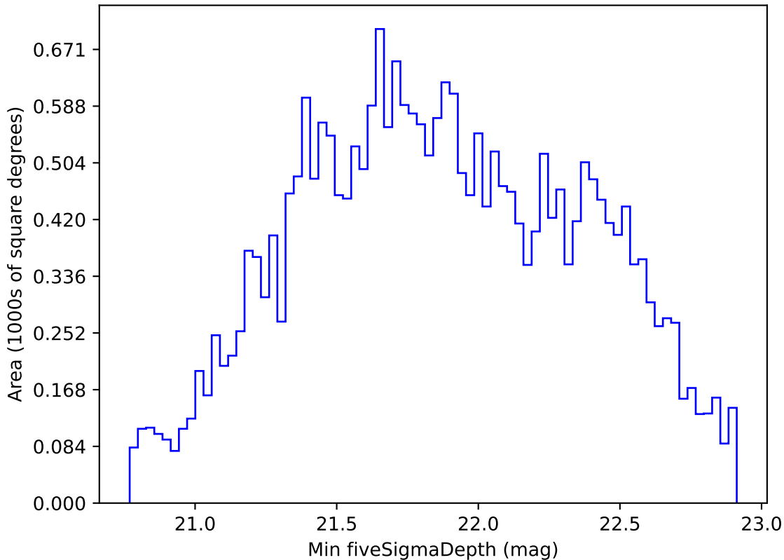
too_combined_s0.5_v3.4_10yrs All sky i band: Min fiveSigmaDepth
