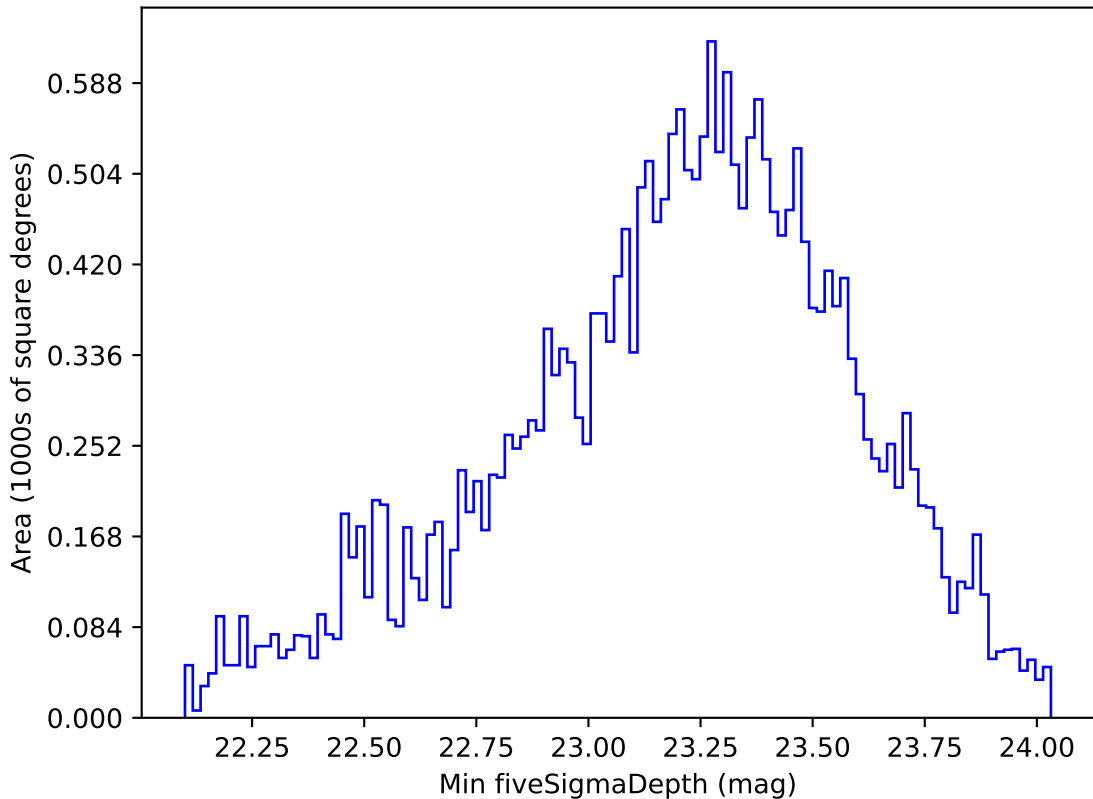
too_combined_s0.5_v3.4_10yrs All sky g band: Min fiveSigmaDepth
