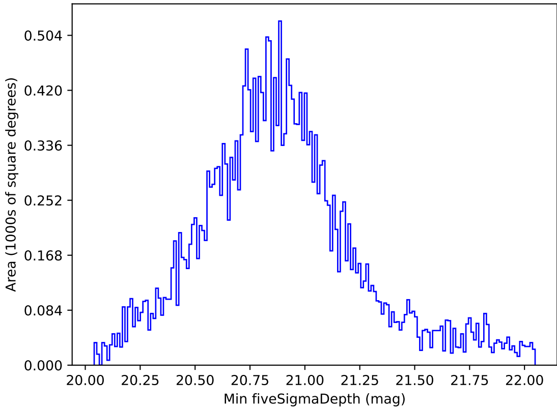
too_combined_s0.5_v3.4_10yrs All sky all bands: Min fiveSigmaDepth
