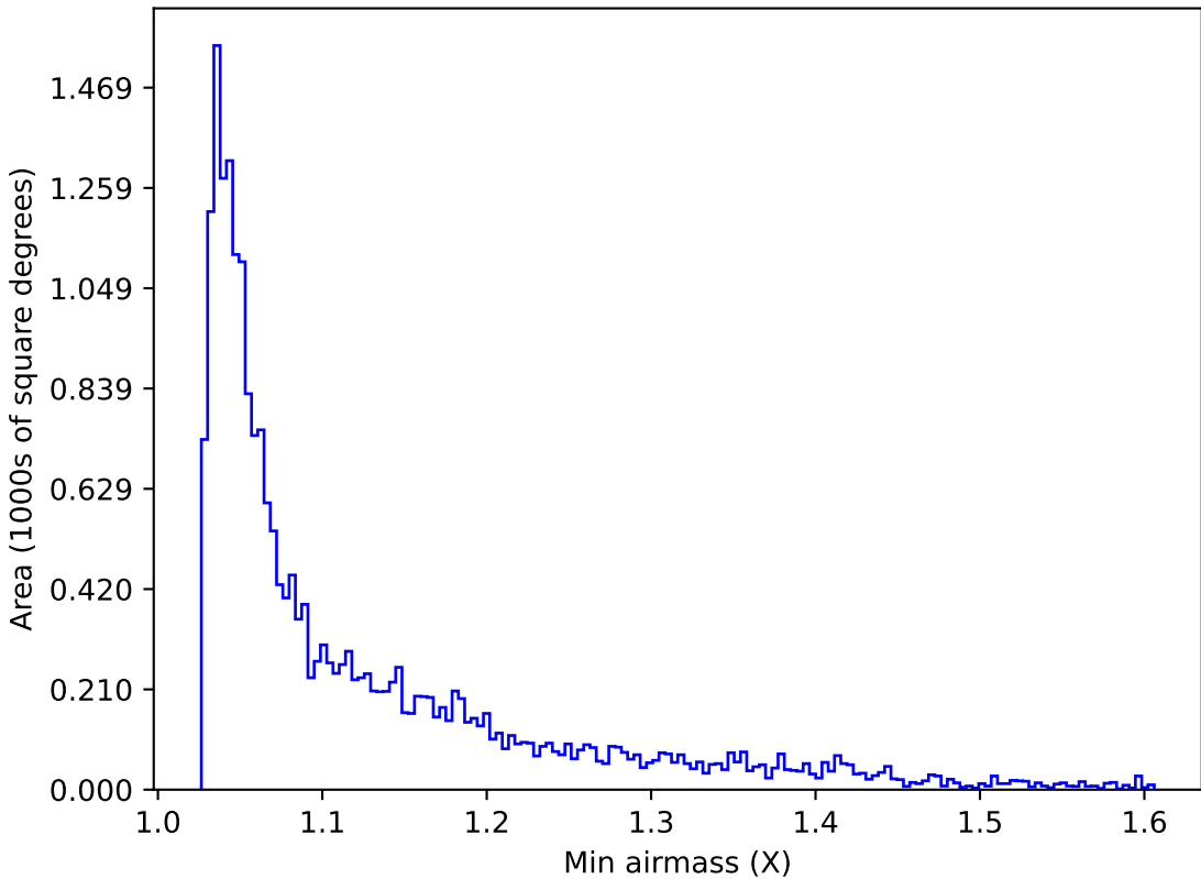
too_combined_s0.5_v3.4_10yrs Yr 1 y band: Min airmass
