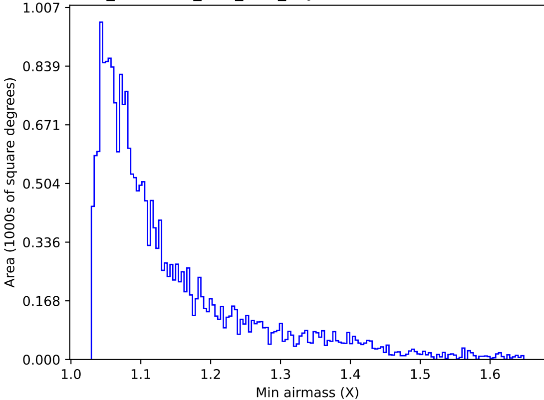
too_combined_s0.5_v3.4_10yrs Yr 1 u band: Min airmass
