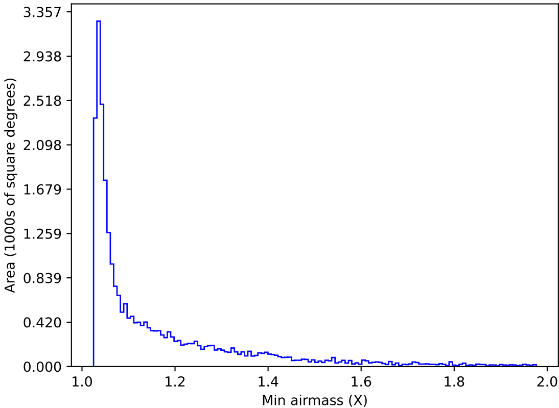
too_combined_s0.5_v3.4_10yrs Yr 1 i band: Min airmass
