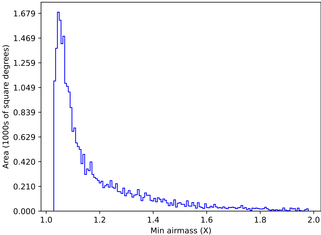
too_combined_s0.5_v3.4_10yrs Yr 1 g band: Min airmass
