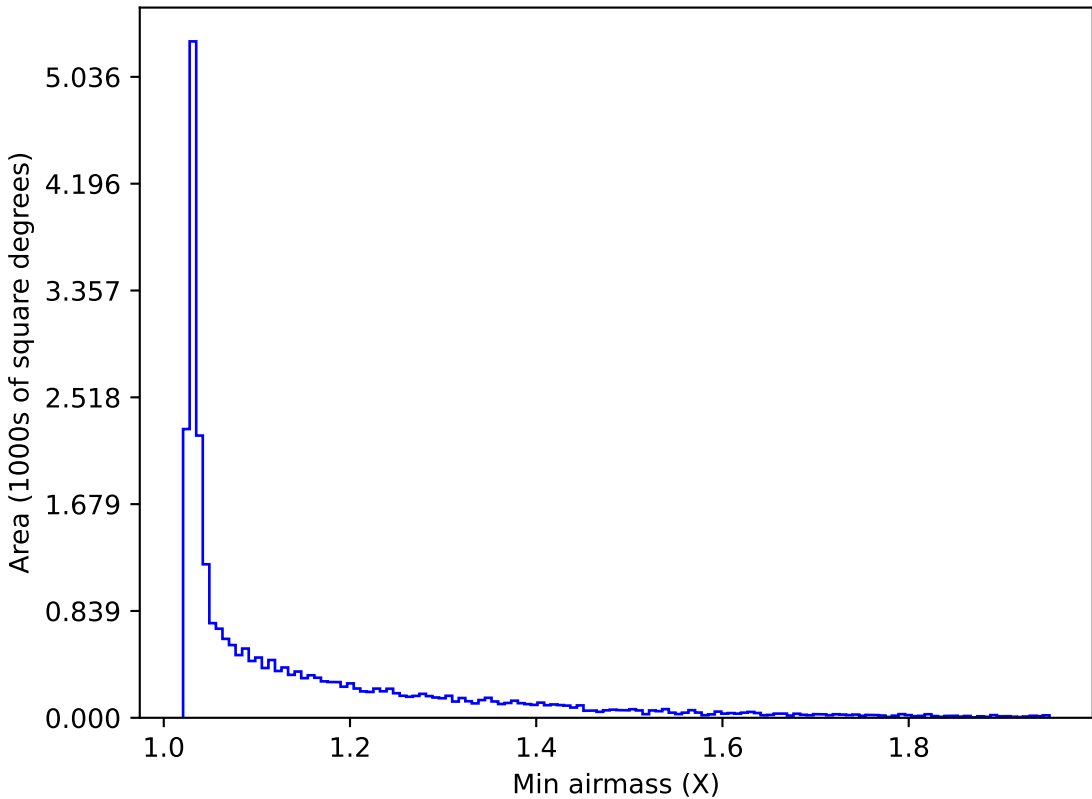
too_combined_s0.5_v3.4_10yrs Yr 1 all bands: Min airmass
