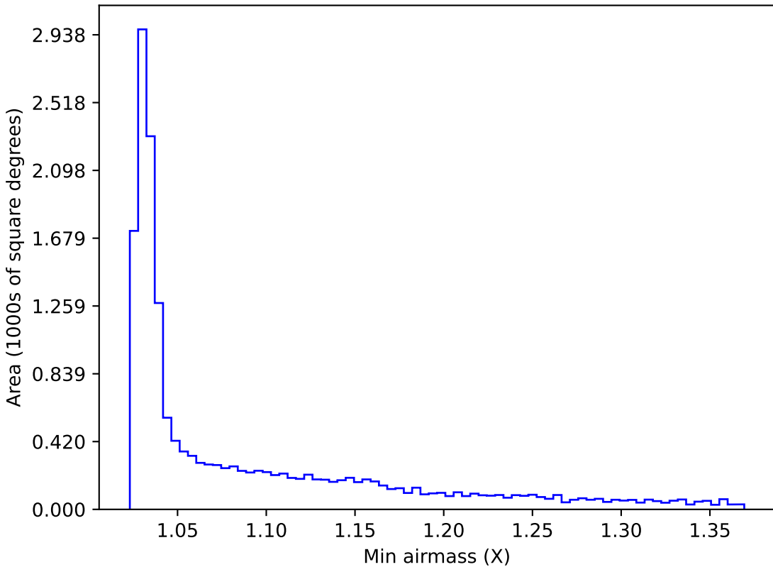
too_combined_s0.5_v3.4_10yrs WFD y band: Min airmass
