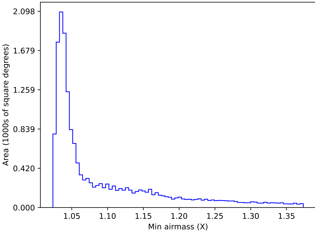
too_combined_s0.5_v3.4_10yrs WFD u band: Min airmass
