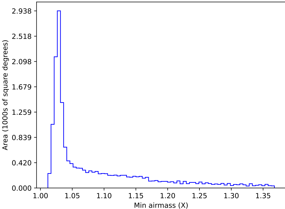
too_combined_s0.5_v3.4_10yrs WFD r band: Min airmass
