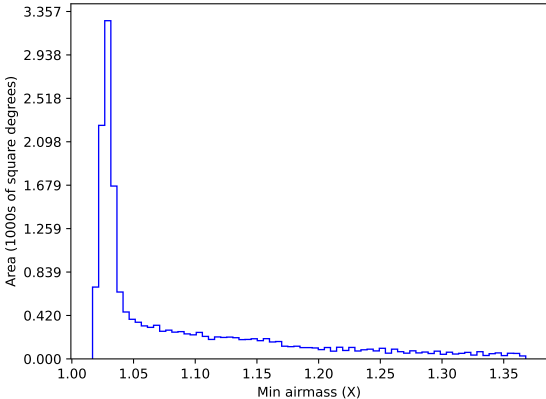
too_combined_s0.5_v3.4_10yrs WFD i band: Min airmass
