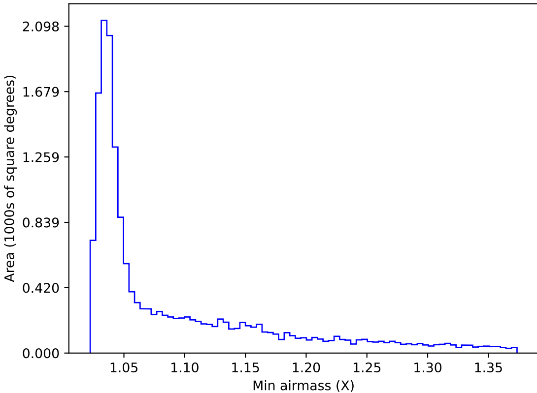
too_combined_s0.5_v3.4_10yrs WFD g band: Min airmass
