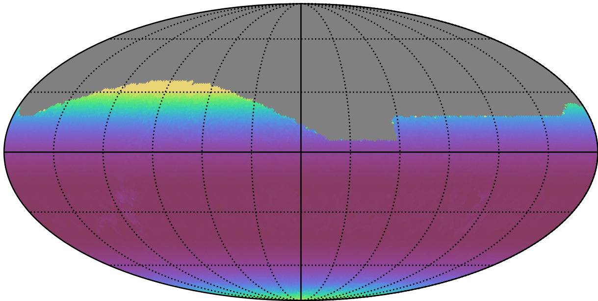
too_combined_s0.5_v3.4_10yrs All sky z band: Min airmass
