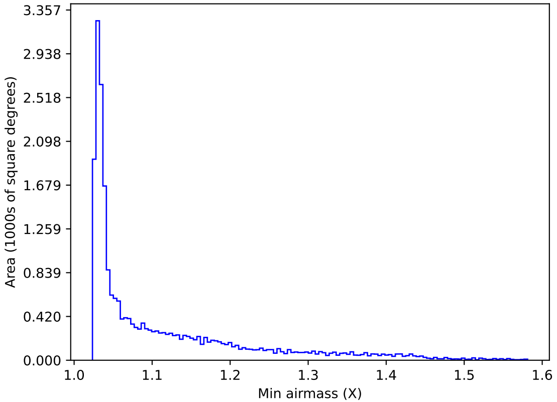
too_combined_s0.5_v3.4_10yrs All sky y band: Min airmass
