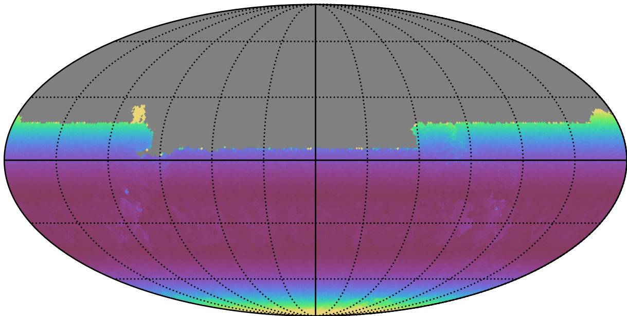
too_combined_s0.5_v3.4_10yrs All sky u band: Min airmass
