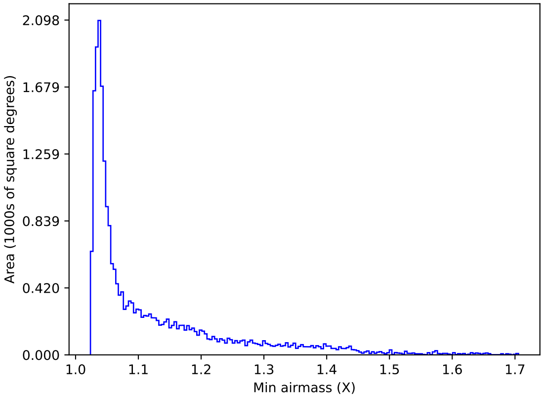
too_combined_s0.5_v3.4_10yrs All sky u band: Min airmass
