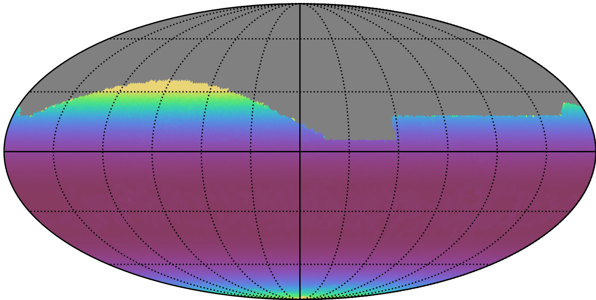
too_combined_s0.5_v3.4_10yrs All sky r band: Min airmass
