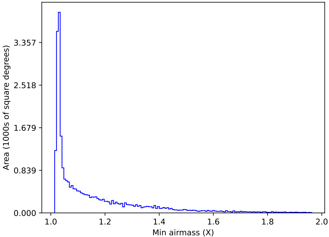
too_combined_s0.5_v3.4_10yrs All sky r band: Min airmass
