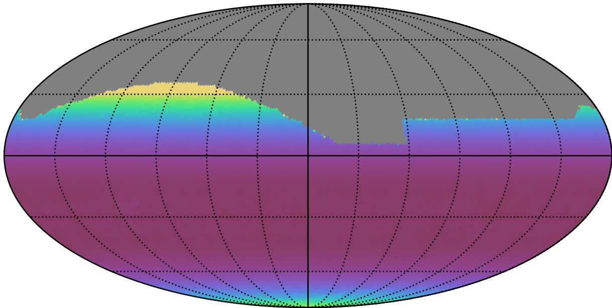
too_combined_s0.5_v3.4_10yrs All sky i band: Min airmass
