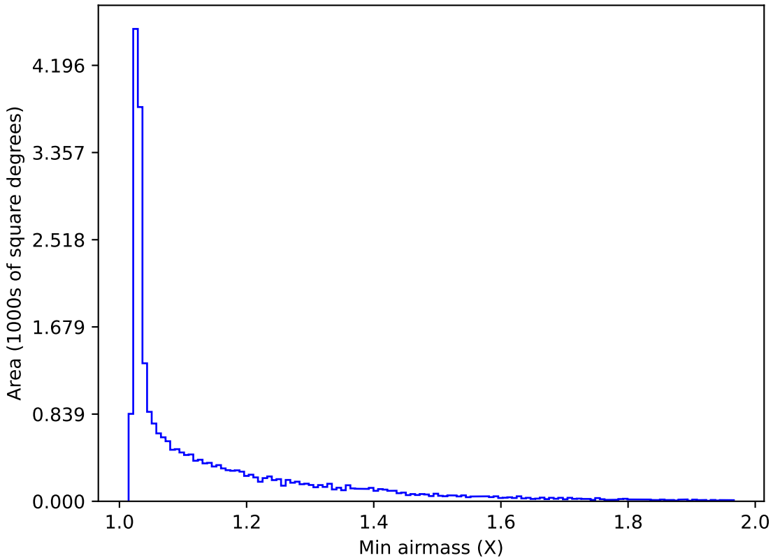
too_combined_s0.5_v3.4_10yrs All sky i band: Min airmass
