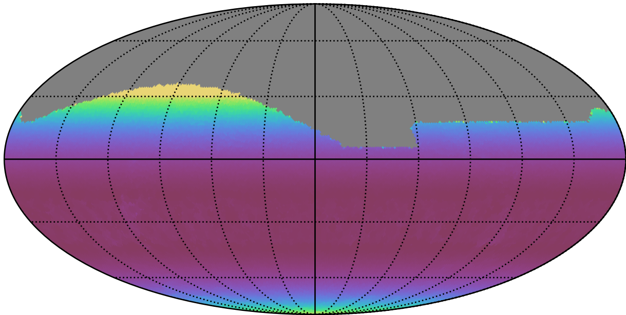
too_combined_s0.5_v3.4_10yrs All sky g band: Min airmass
