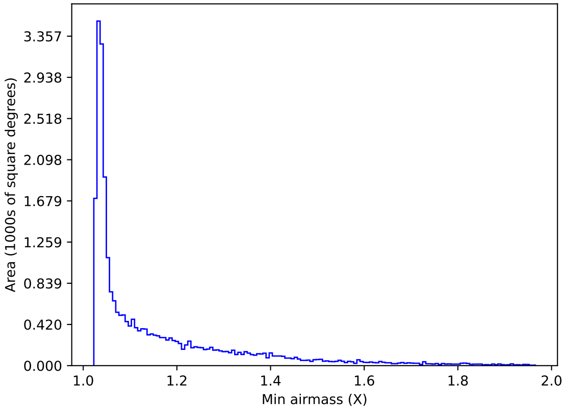
too_combined_s0.5_v3.4_10yrs All sky g band: Min airmass
