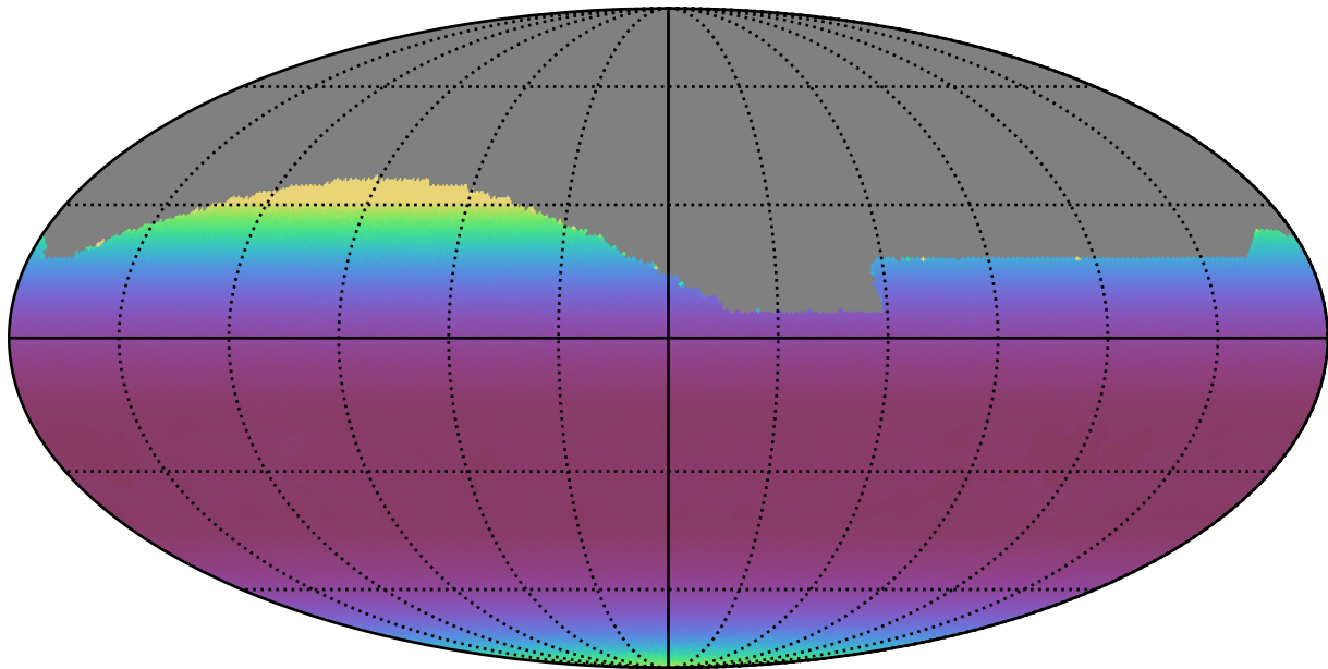
too_combined_s0.5_v3.4_10yrs All sky all bands: Min airmass
