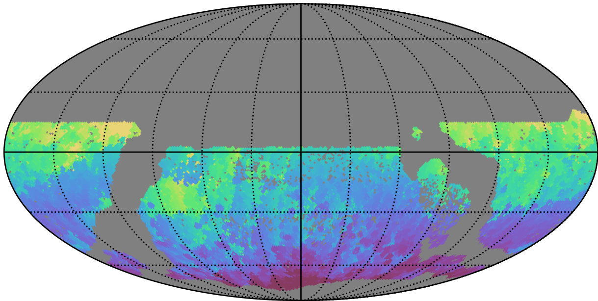
too_combined_s0.5_v3.4_10yrs WFD z band: Min HA
