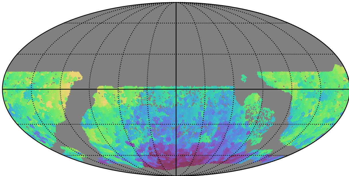
too_combined_s0.5_v3.4_10yrs WFD y band: Min HA
