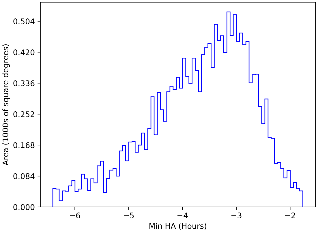
too_combined_s0.5_v3.4_10yrs WFD y band: Min HA
