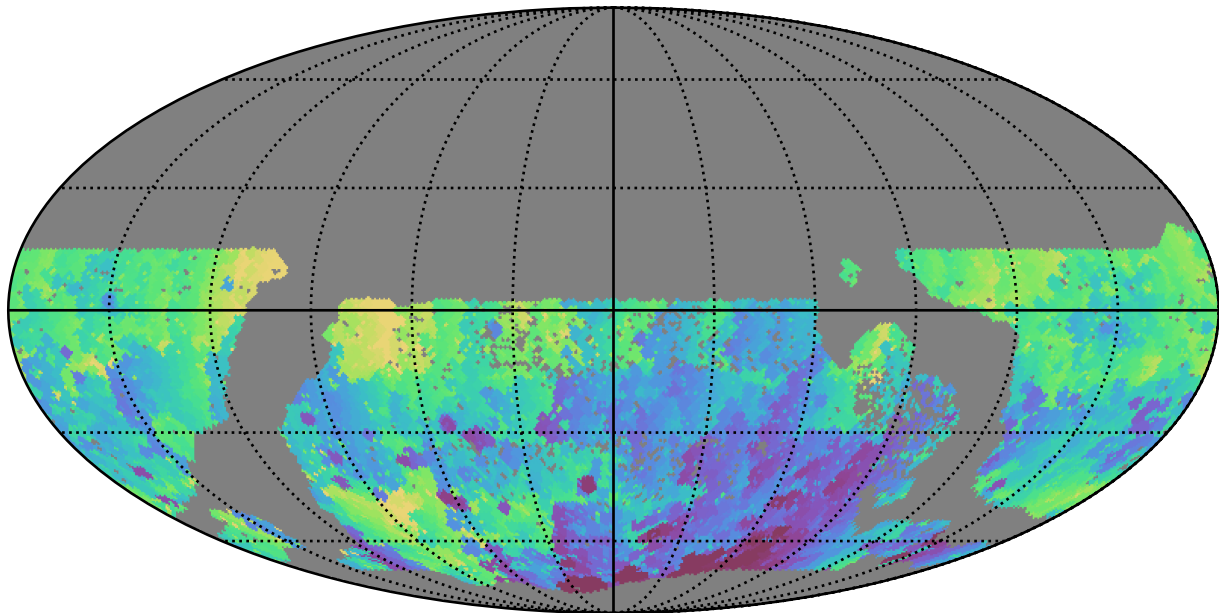
too_combined_s0.5_v3.4_10yrs WFD u band: Min HA
