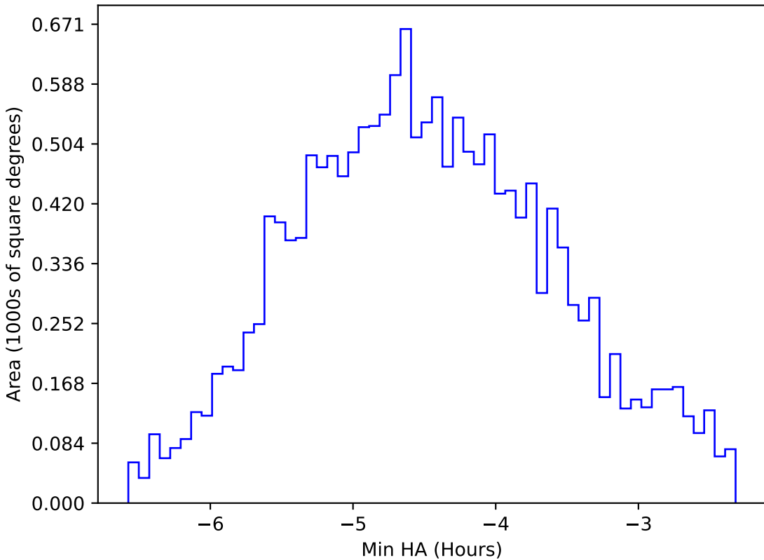
too_combined_s0.5_v3.4_10yrs WFD r band: Min HA
