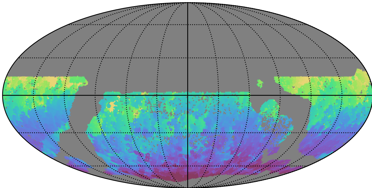
too_combined_s0.5_v3.4_10yrs WFD i band: Min HA
