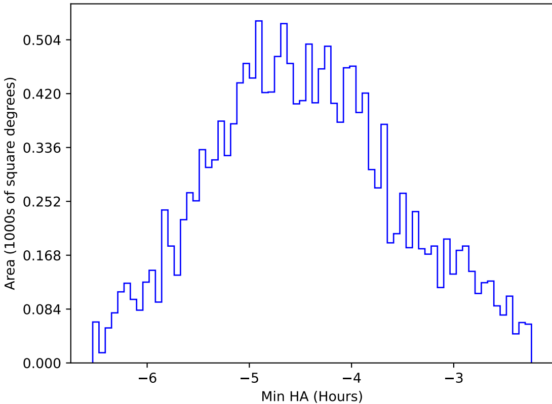
too_combined_s0.5_v3.4_10yrs WFD i band: Min HA
